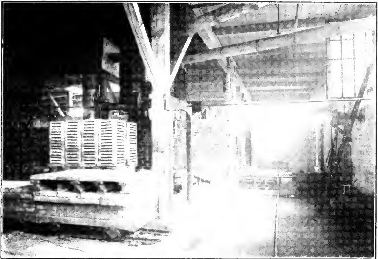
The Charge End of the Tunnel Kiln Type of Furnace. An empty and a loaded truck are seen in the left foreground
